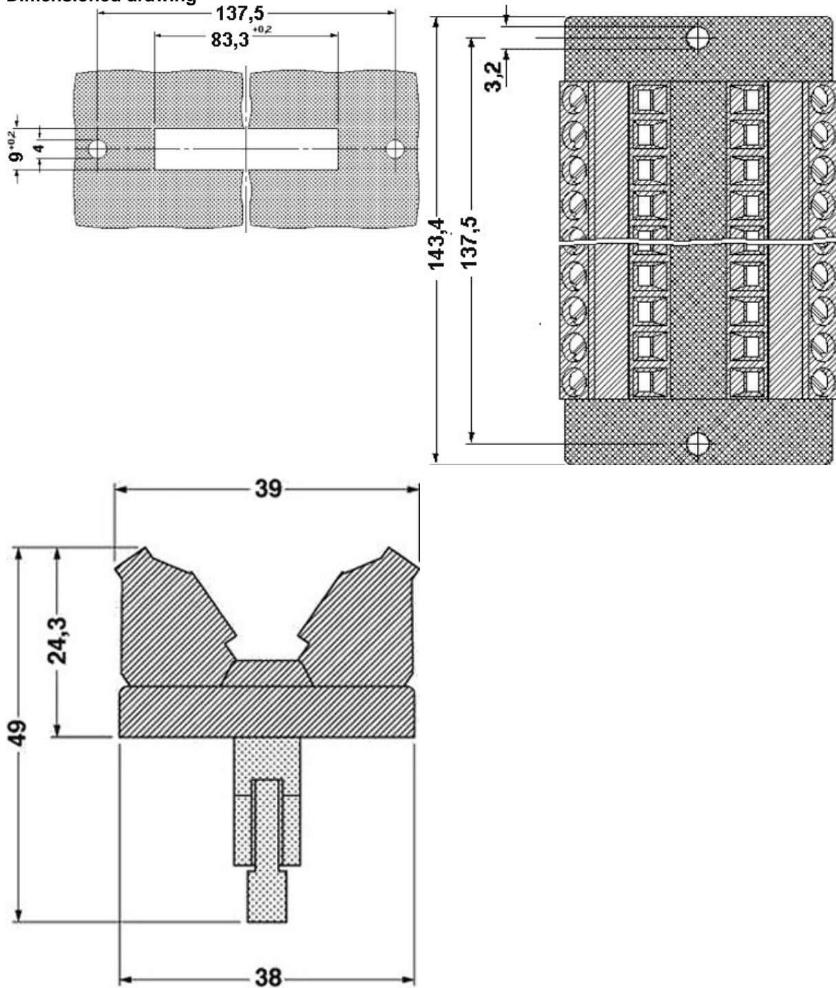
Dimensioned drawing
